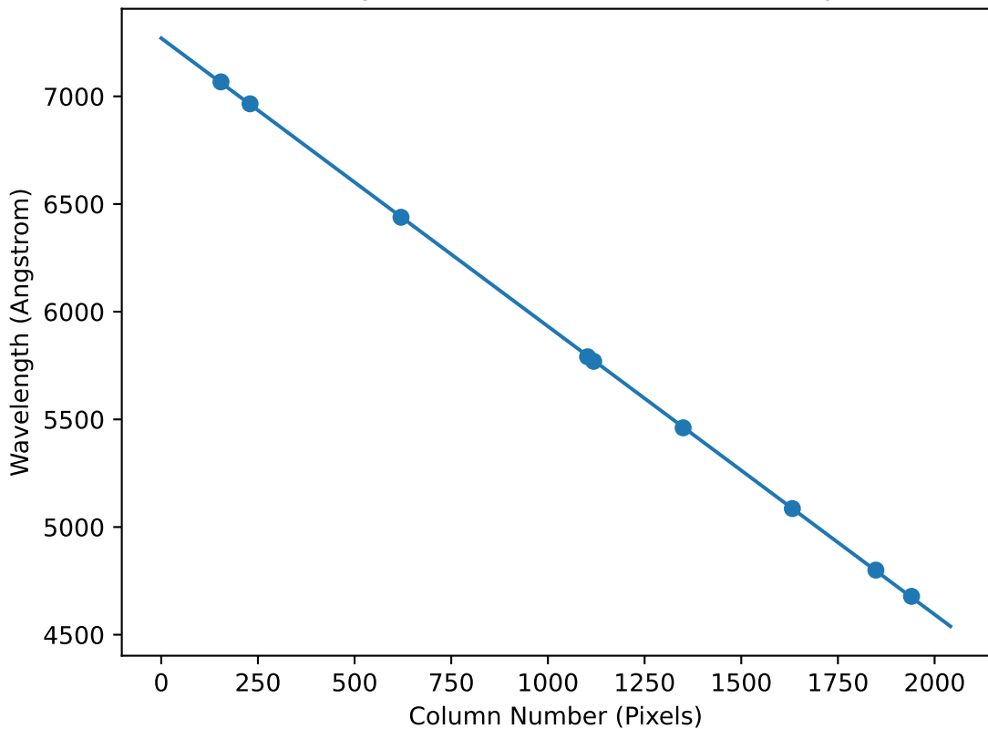
Wavelength Calibration Function Fit Analysis
